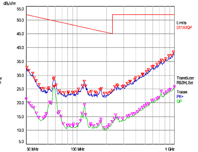
Radiated emissions 30 – 1000 MHz @ 110 Vin horizontal polarization
