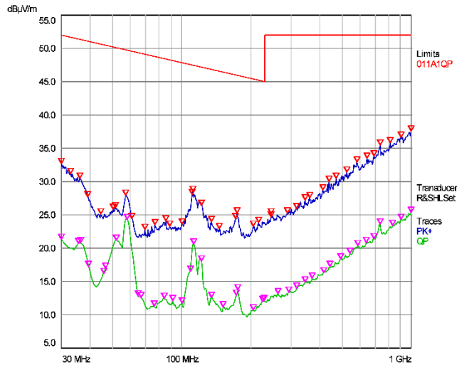
Radiated emissions 30 – 1000 MHz @ 110 Vin vertical polarization
